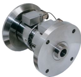
Stamicco extrusion melt blender SMB-R with housing
